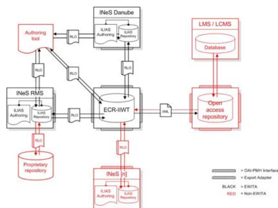
Figure 3: Architecture Content Repository
